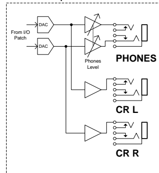
Phones/CR Outputs
